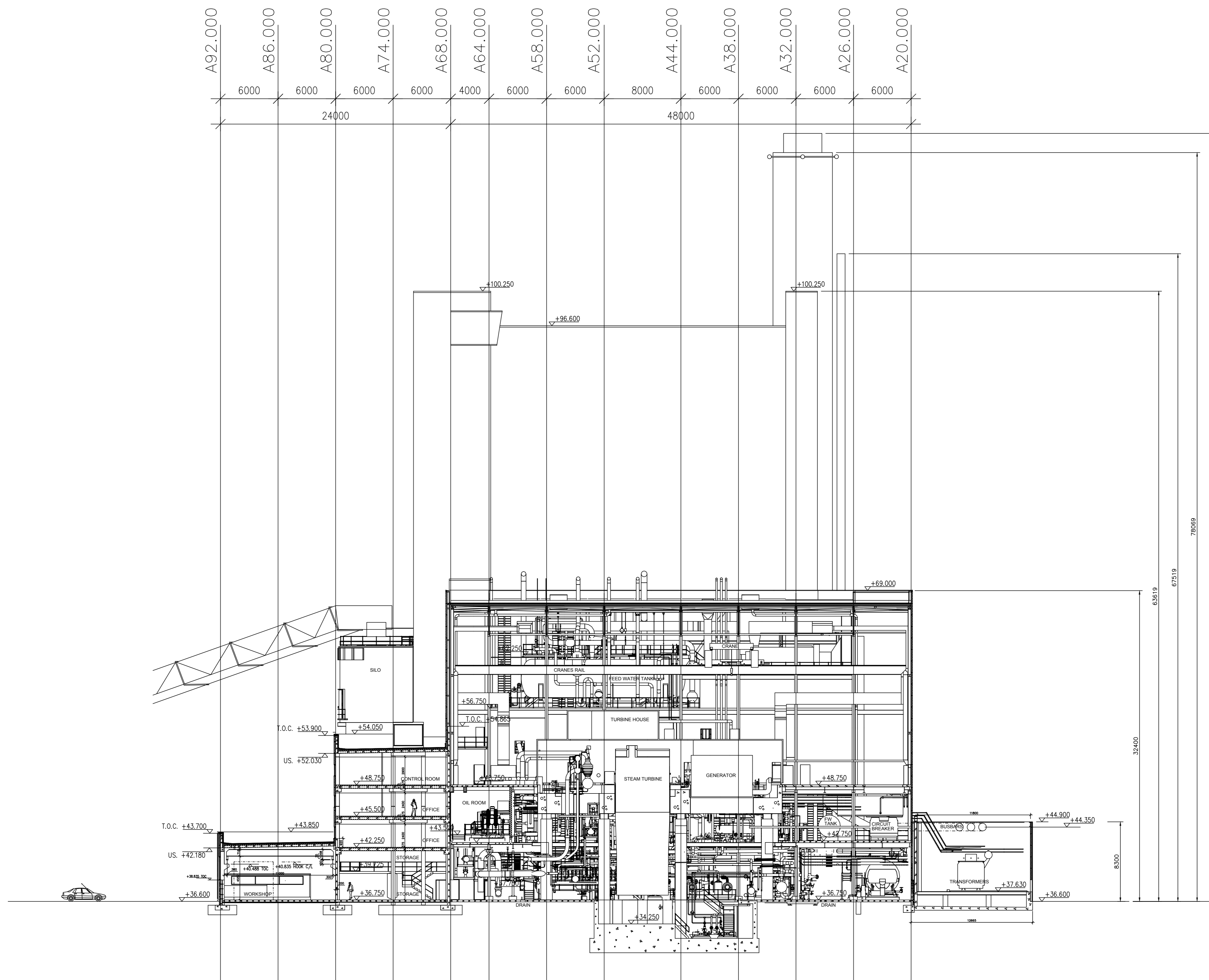
SECTION B-B @ 1:200 (REFER TO DRGS. QS-000263-01-D460-058 TO 060)
